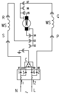
Electric Circuit
