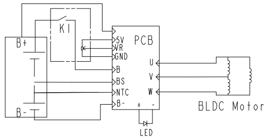
Electric Circuit
